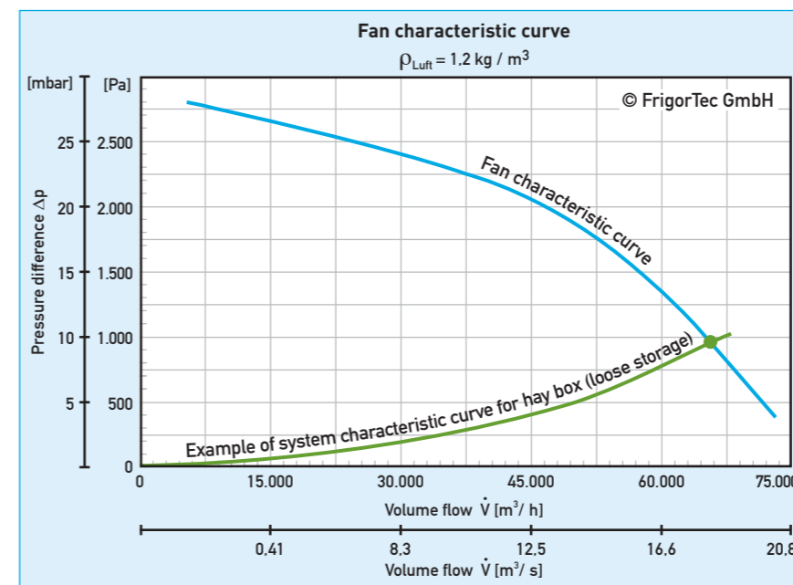
20 Characteristic curve of an AGRIFRIGOR™ fan
