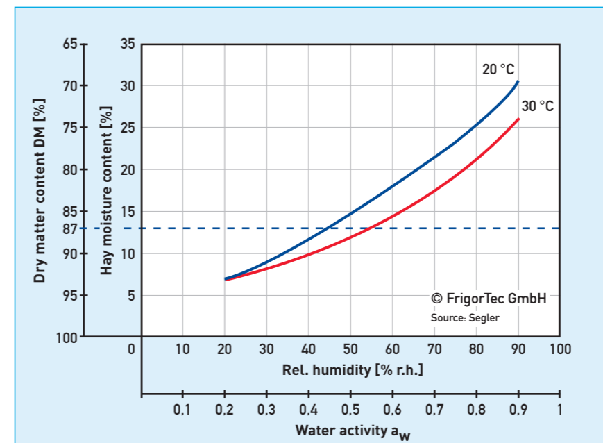
21 Sorption isotherms of hay
