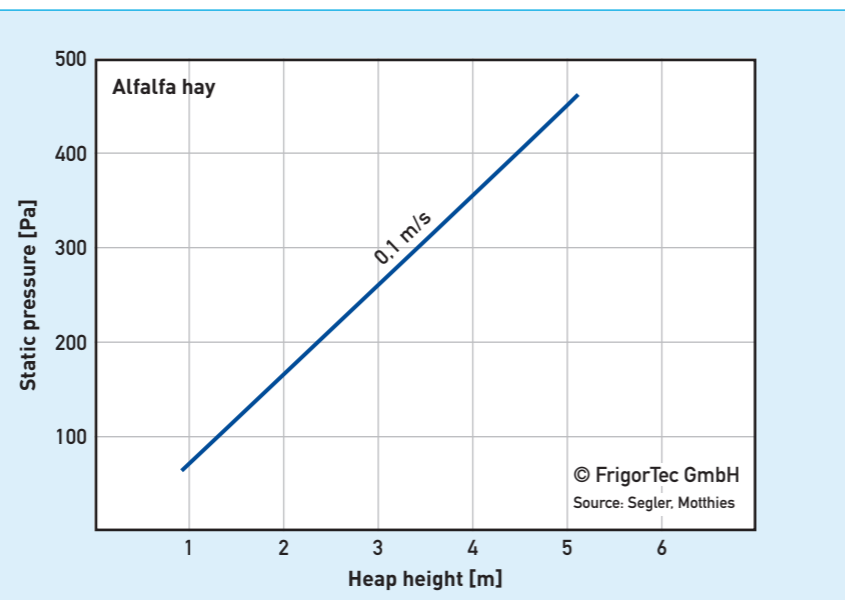
18 Pressure loss with alfalfa hay (6)
